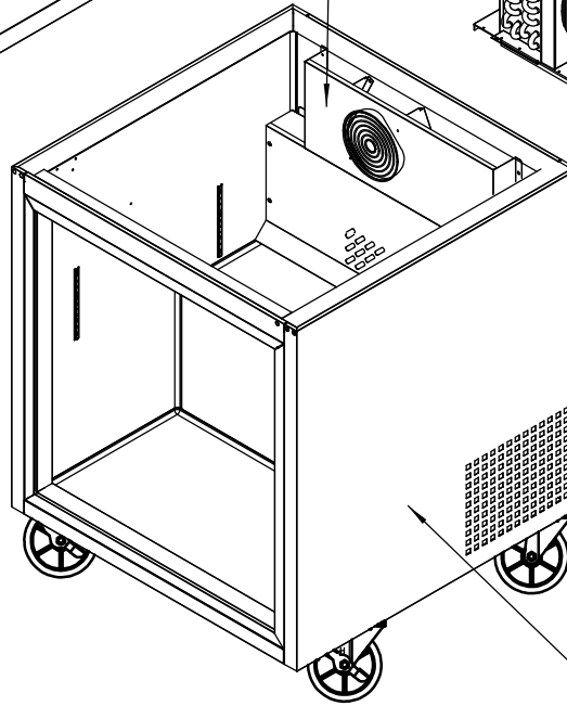
CABINET ASSEMBLY PART D
