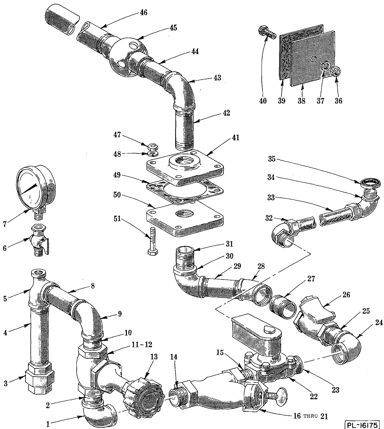
STEAM INJECTOR
