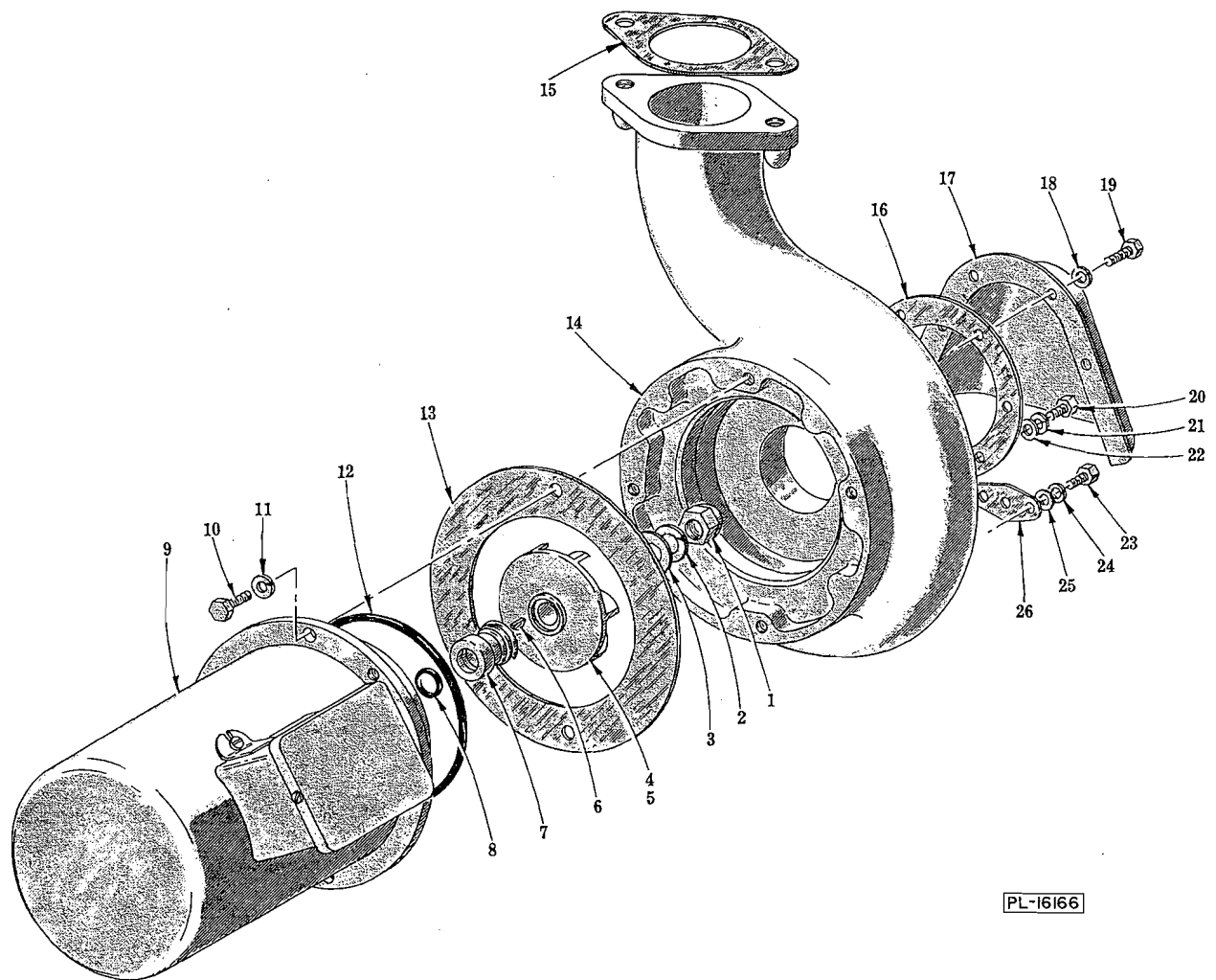
AM-12A MOTOR AND PUMP UNIT
