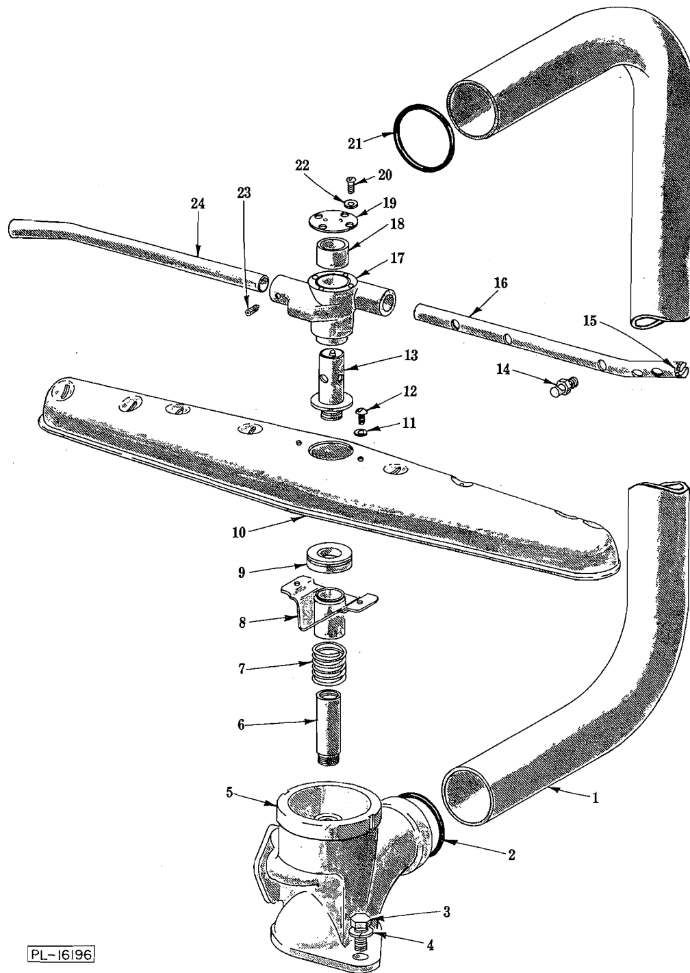
LOWER WASH ARM UNIT
