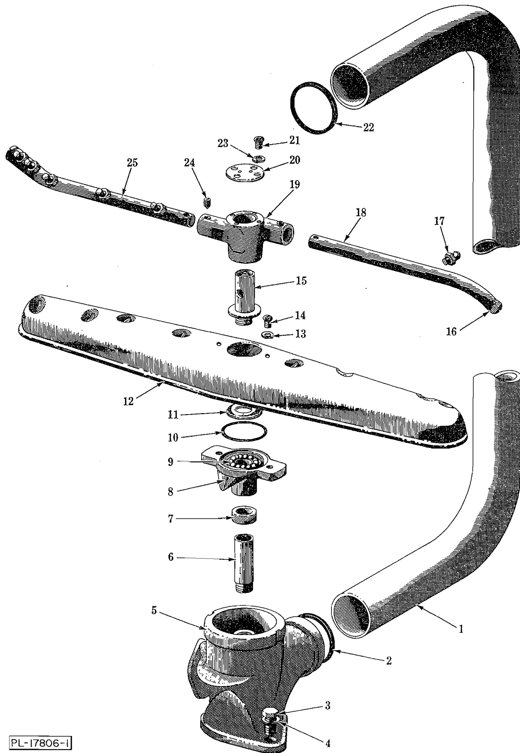
LOWER WASH ARM UNIT
