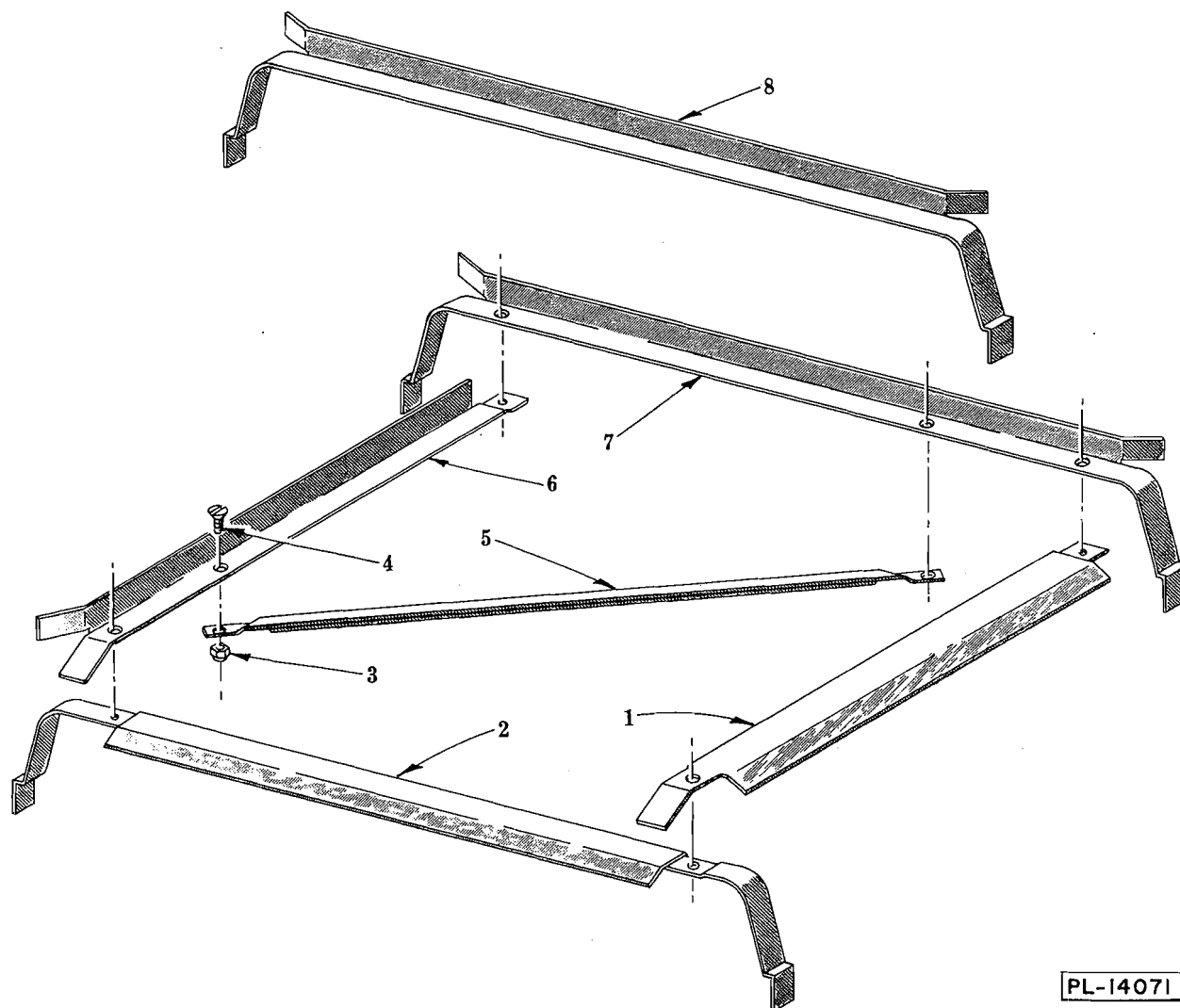
TRACK UNIT
