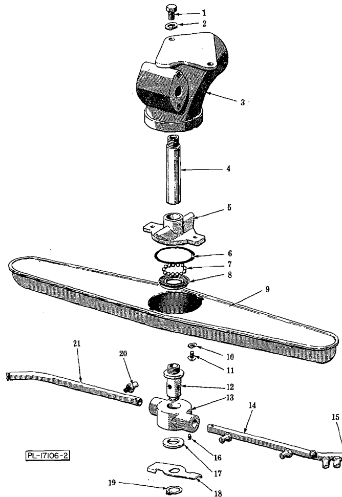
UPPER WASH ARM UNIT (BALL BEARING TYPE) (WITH ROTATING RINSE)
