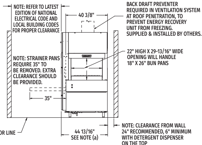
Back/Unload End
