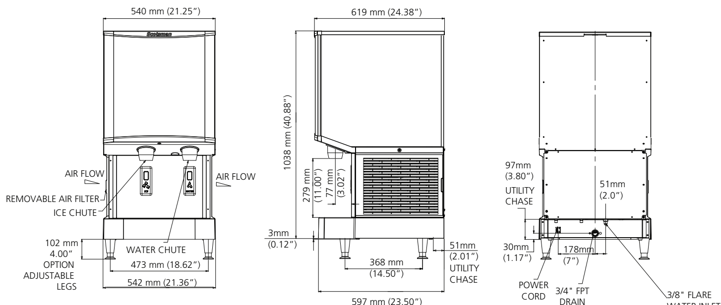
FRONT VIEW
