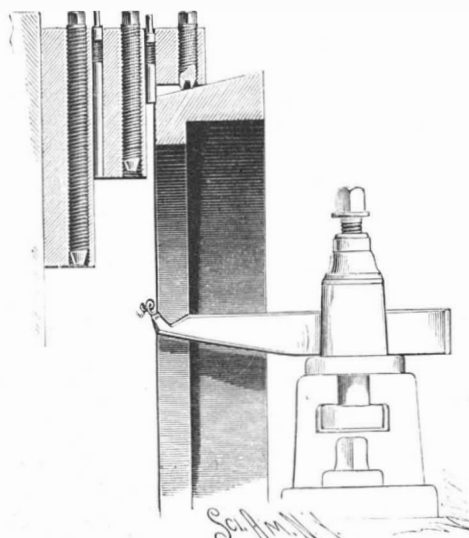
IDE'S LATHE CHUCK.
