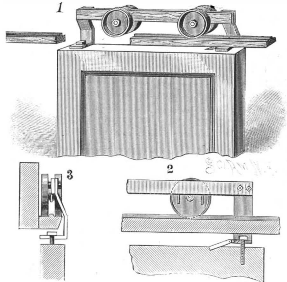
SMITH'S DOOR HANGER.
